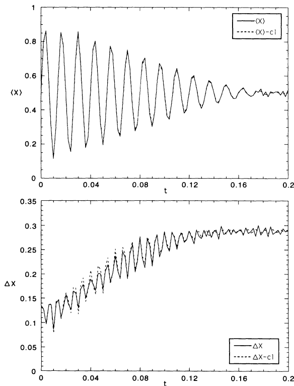
FIG. 3. Average and rms half-width of the position probability distribution for a non-Gaussian state with mean velocity v=150 , according to quantum (solid line) and classical theories (dotted line).
