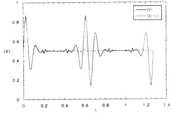
FIG. 1. Average position for a particle confined to the unit interval, according to quantum theory (solid line) and classical ensemble theory (dotted line). The initial state is Gaussian with half-width a = 0.1 and mean velocity v = 20 .
