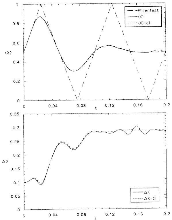
FIG. 2. Upper half: average position according to quantum and classical theories compared with Ehrenfest's theorem (sawtooth curve). Lower half: rms half-width of the position probability distribution, according to quantum (solid line) and classical theories (dotted line).
