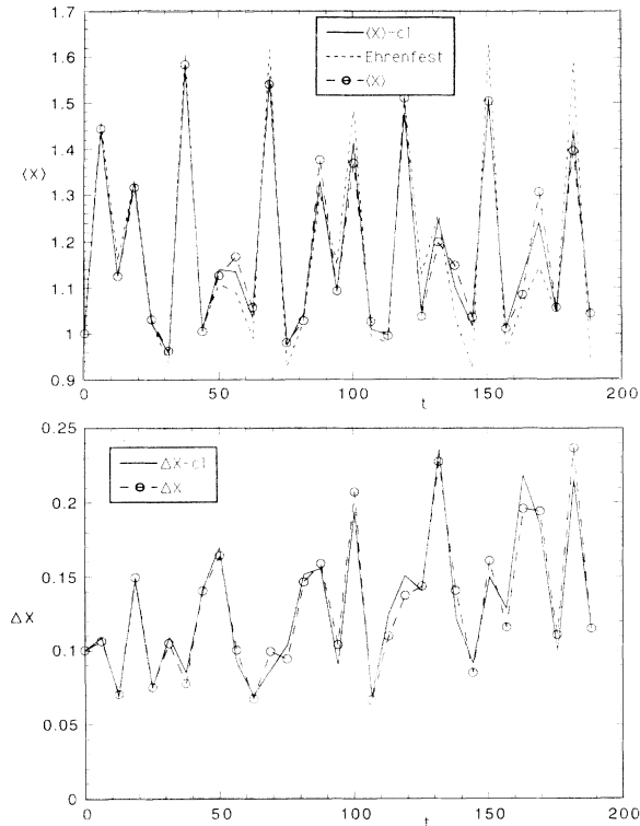
FIG. 5. Driven quartic oscillator in a classically regular state. (Details as in Fig. 4.)
