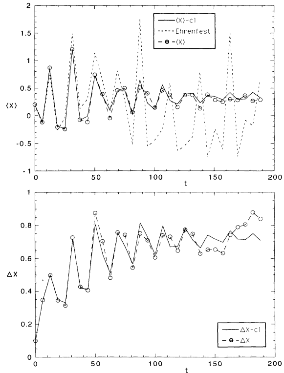
FIG. 4. Driven quartic oscillator in a classically chaotic state. Upper half: average position according to quantum (circles) and classical theories (solid line), compared with Ehrenfest's theorem (dotted line). Lower half: rms half-width of the position probability distribution, according to quantum (circles) and classical theories (solid line).
